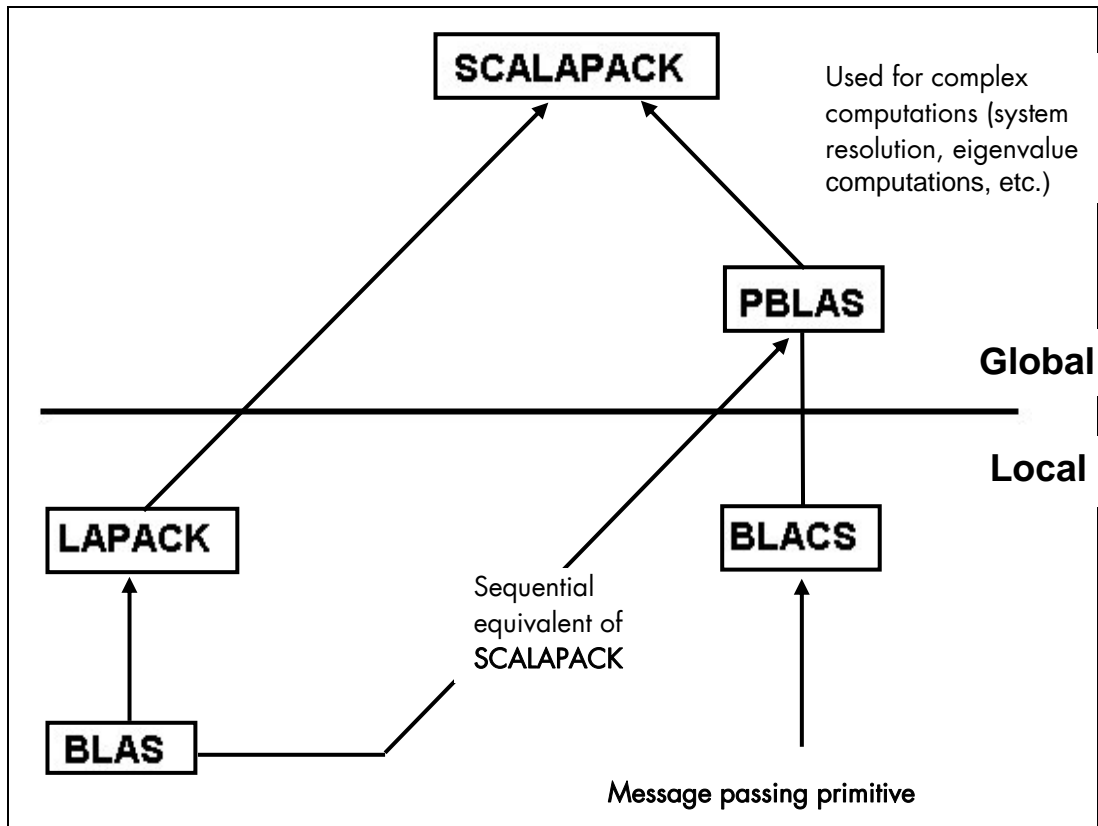
Figure 3-2. Interdependence of the different mathematical libraries (Scientific Studio and Intel)
